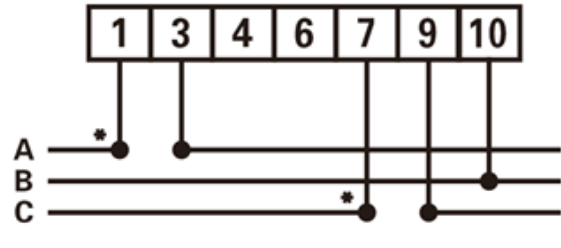
Three phase three wire: direct connect
